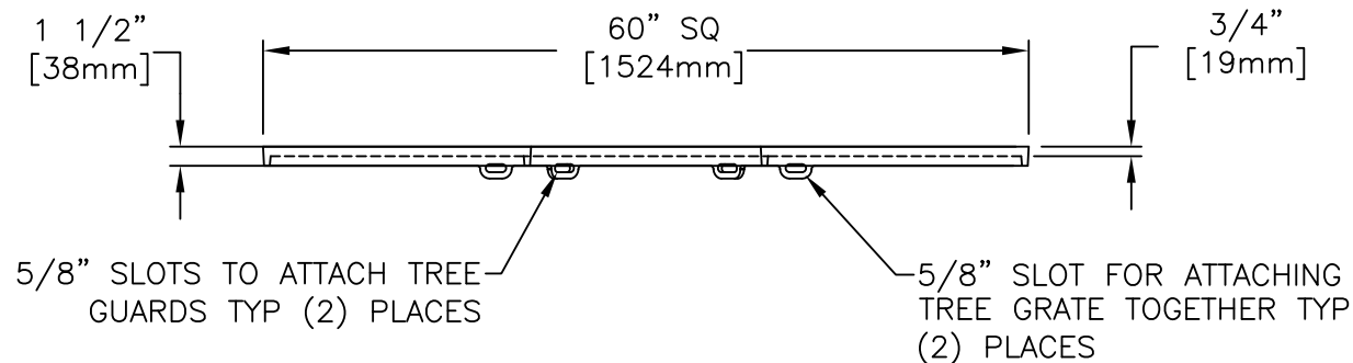
GRATE SECTION
